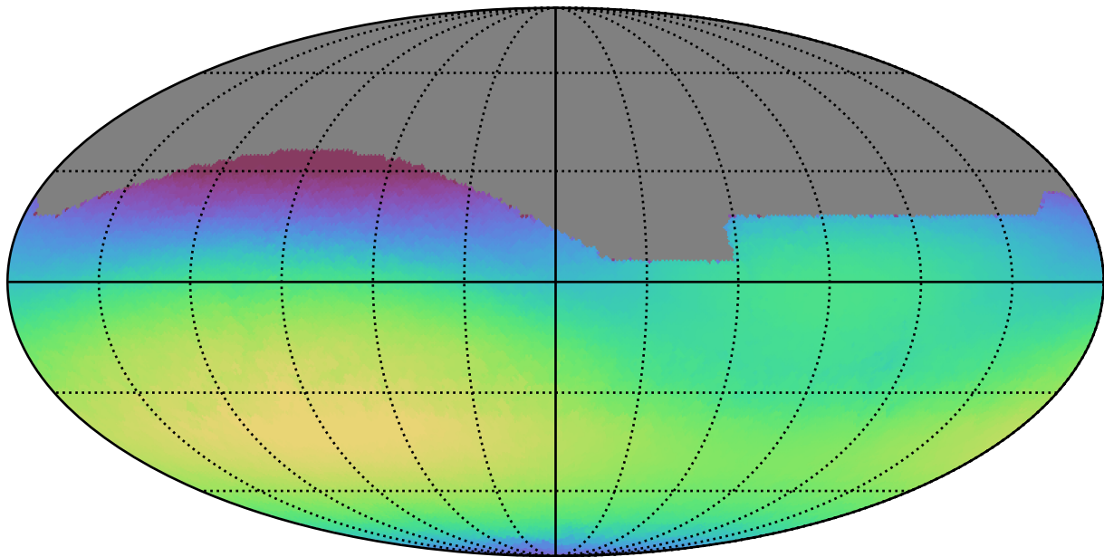
baseline_v2.1_10yrs All sky r band: Max skyBrightness
