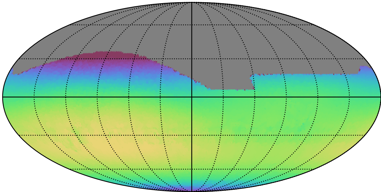
baseline_v2.1_10yrs All sky i band: Max skyBrightness
