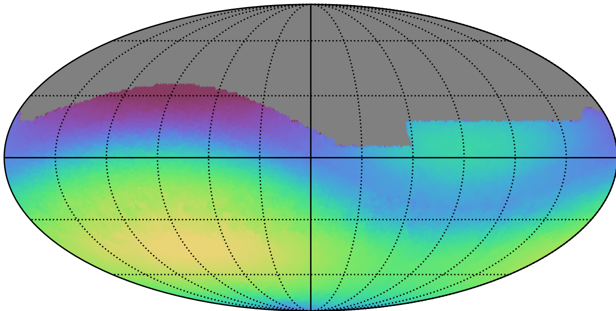
baseline_v2.1_10yrs All sky g band: Max skyBrightness
