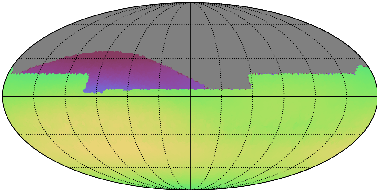
baseline_v2.1_10yrs All sky all bands: Max skyBrightness
