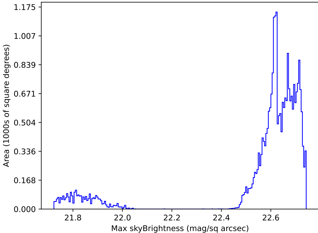
baseline_v2.1_10yrs All sky all bands: Max skyBrightness
