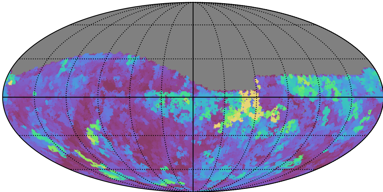
baseline_v2.1_10yrs Yr 1 z band: Max seeingGeom
