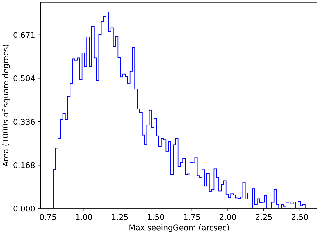
baseline_v2.1_10yrs Yr 1 z band: Max seeingGeom
