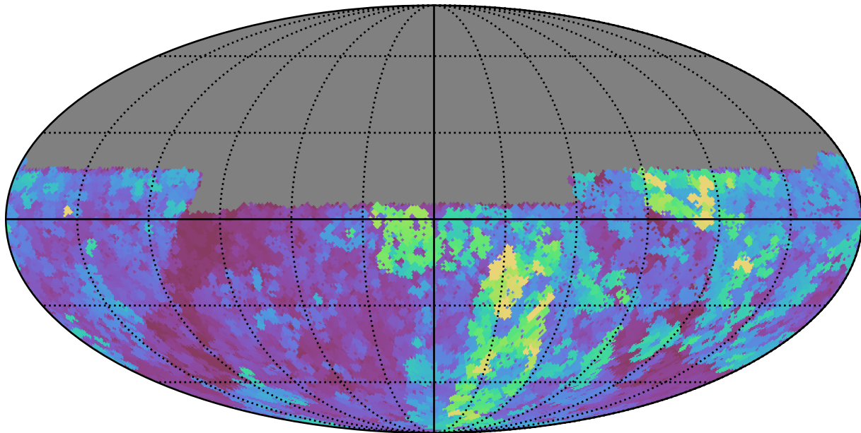
baseline_v2.1_10yrs Yr 1 y band: Max seeingGeom
