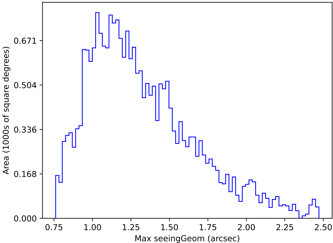
baseline_v2.1_10yrs Yr 1 y band: Max seeingGeom
