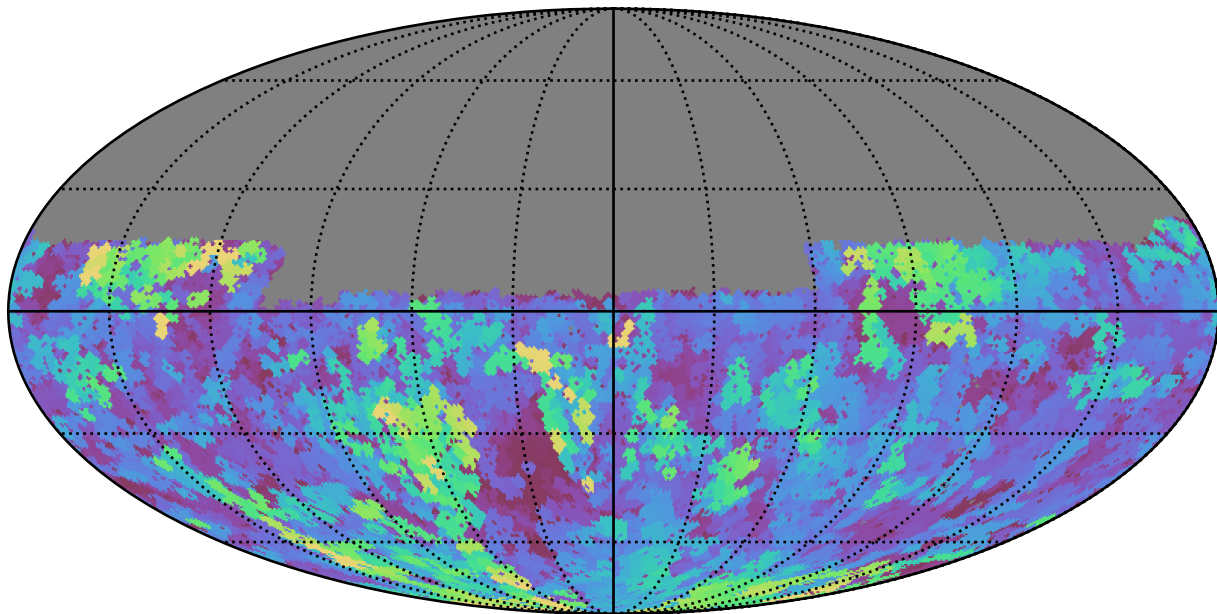
baseline_v2.1_10yrs Yr 1 u band: Max seeingGeom
