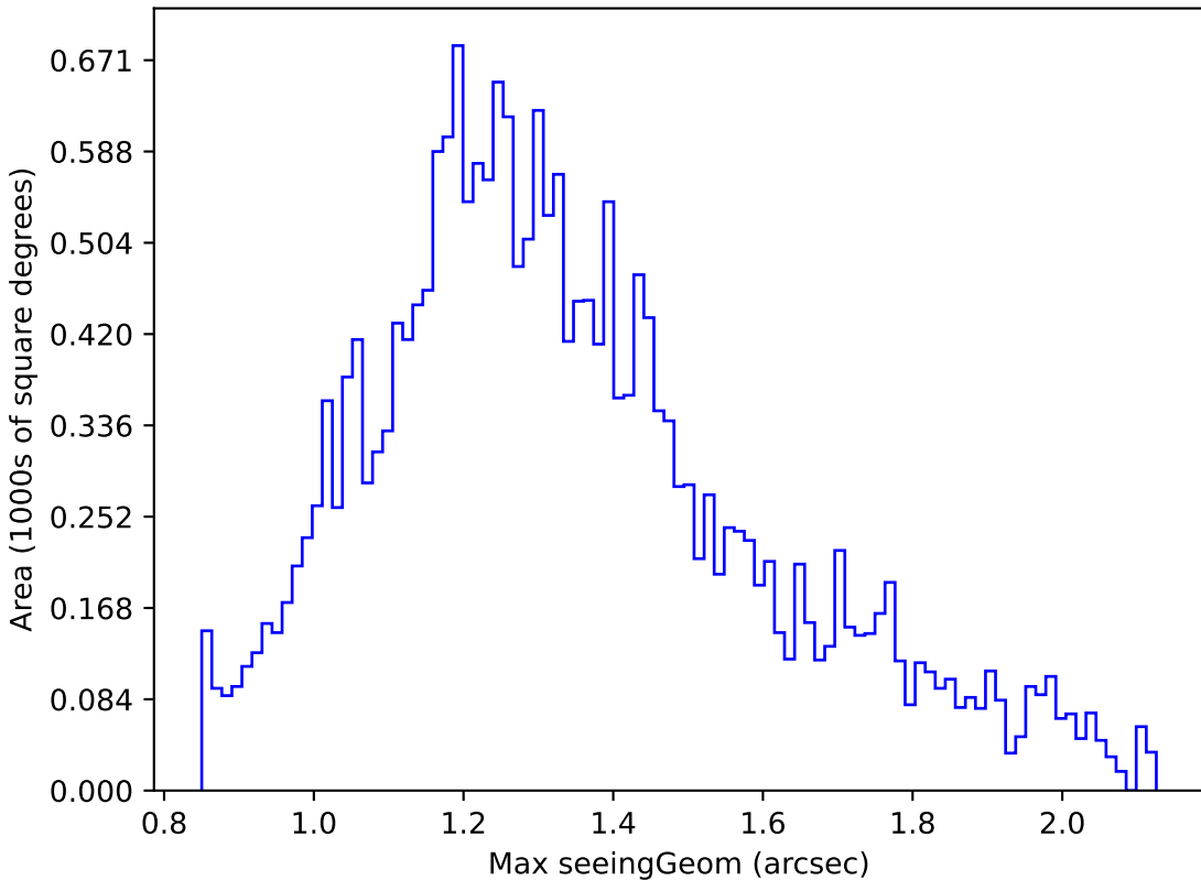
baseline_v2.1_10yrs Yr 1 u band: Max seeingGeom
