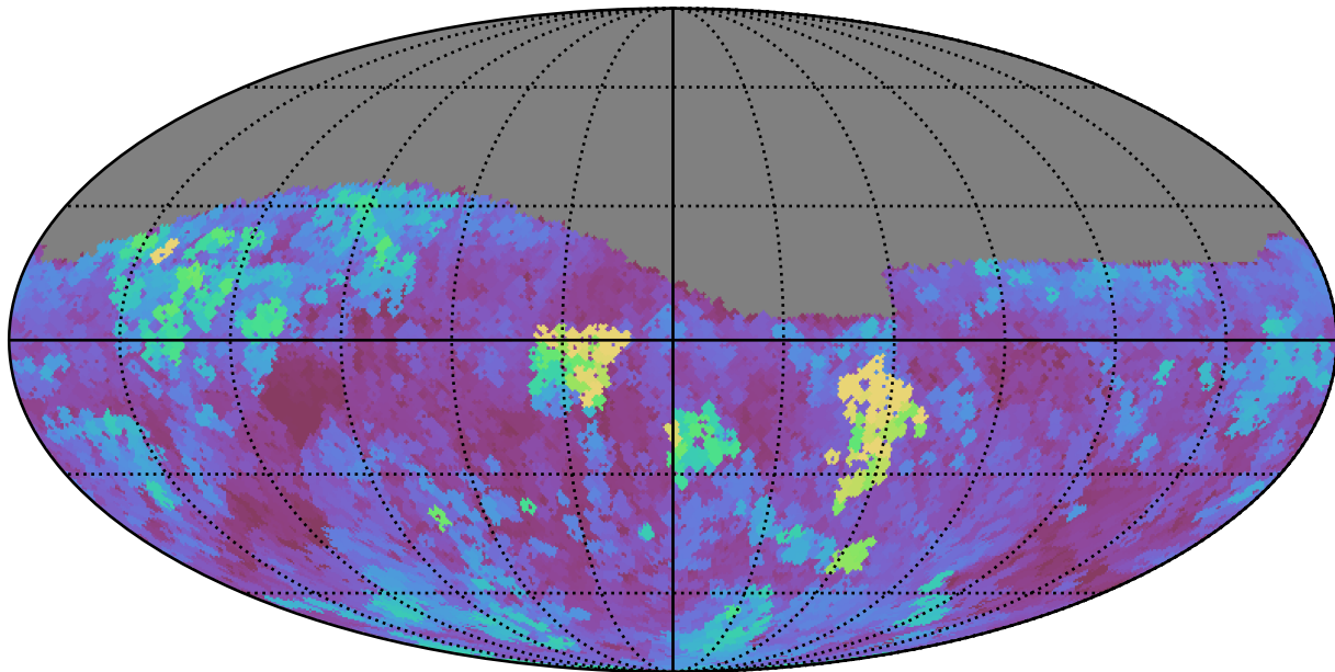
baseline_v2.1_10yrs Yr 1 r band: Max seeingGeom
