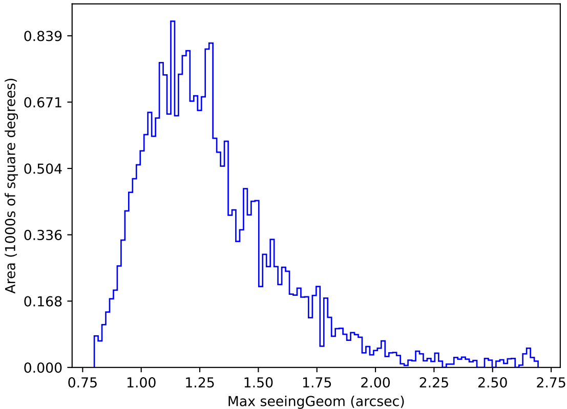
baseline_v2.1_10yrs Yr 1 r band: Max seeingGeom
