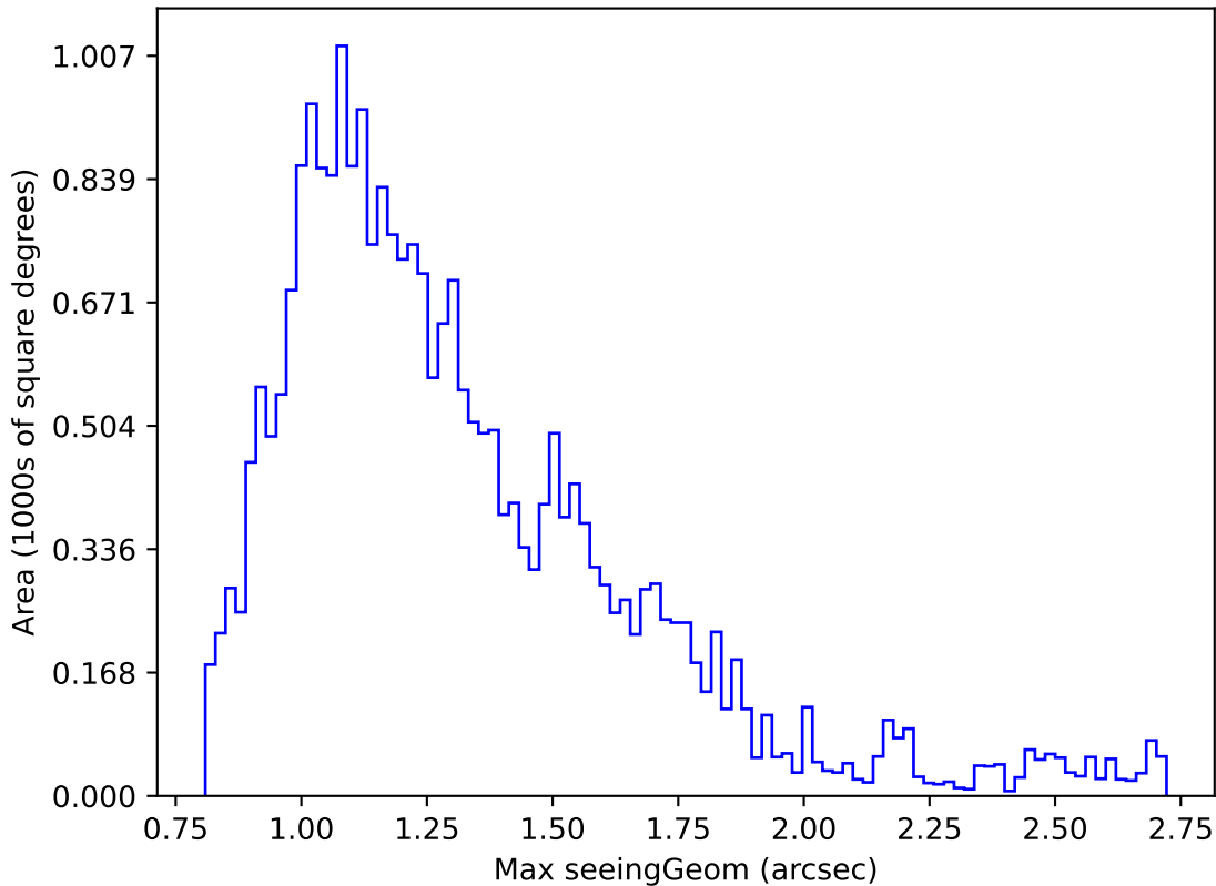
baseline_v2.1_10yrs Yr 1 i band: Max seeingGeom
