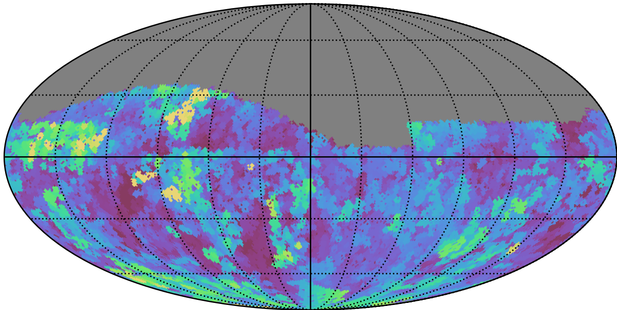
baseline_v2.1_10yrs Yr 1 g band: Max seeingGeom
