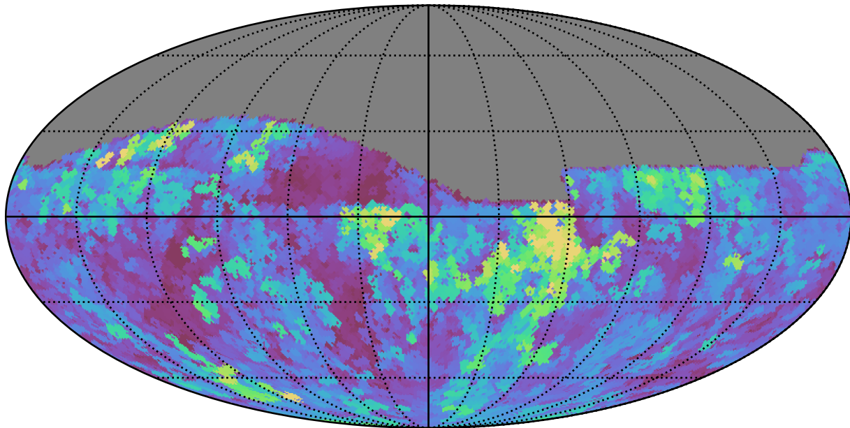
baseline_v2.1_10yrs Yr 1 all bands: Max seeingGeom
