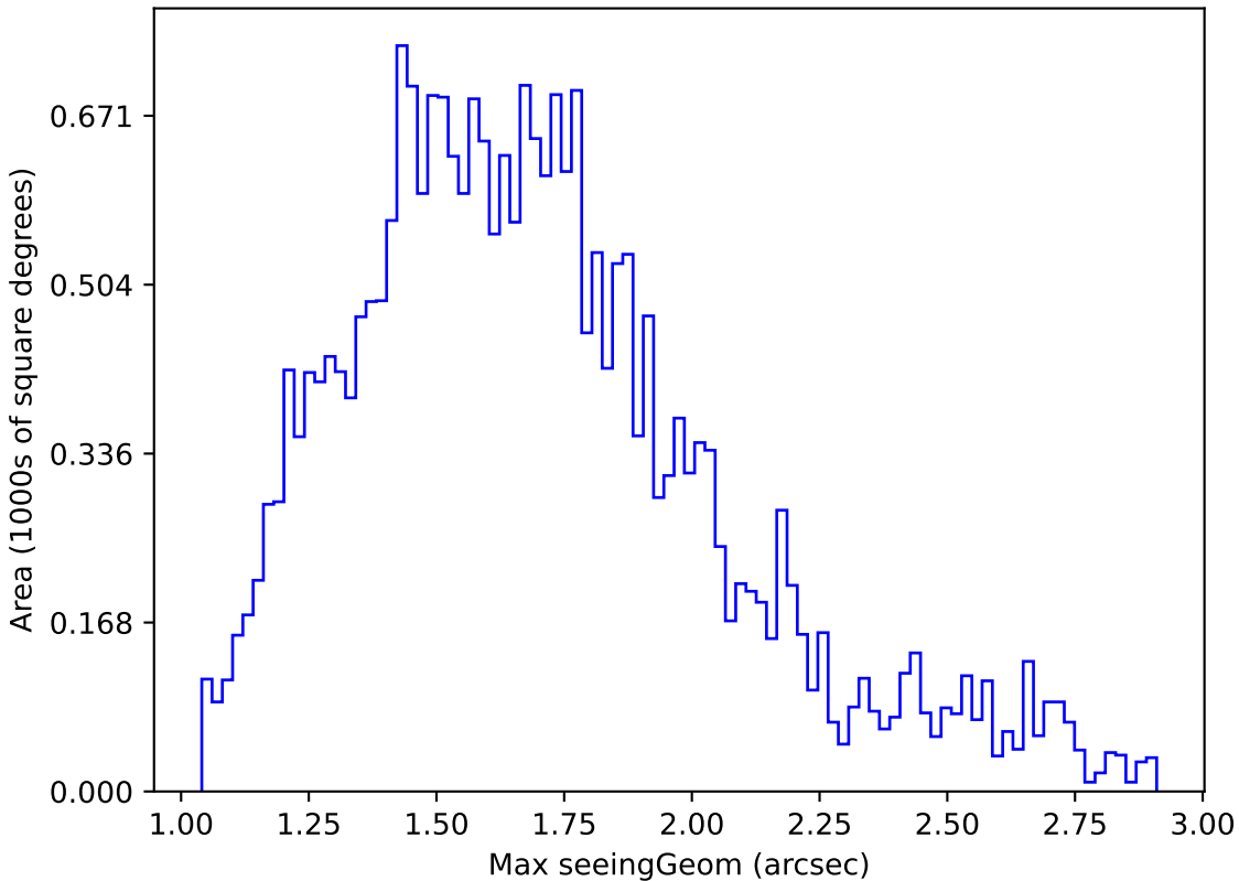
baseline_v2.1_10yrs Yr 1 all bands: Max seeingGeom
