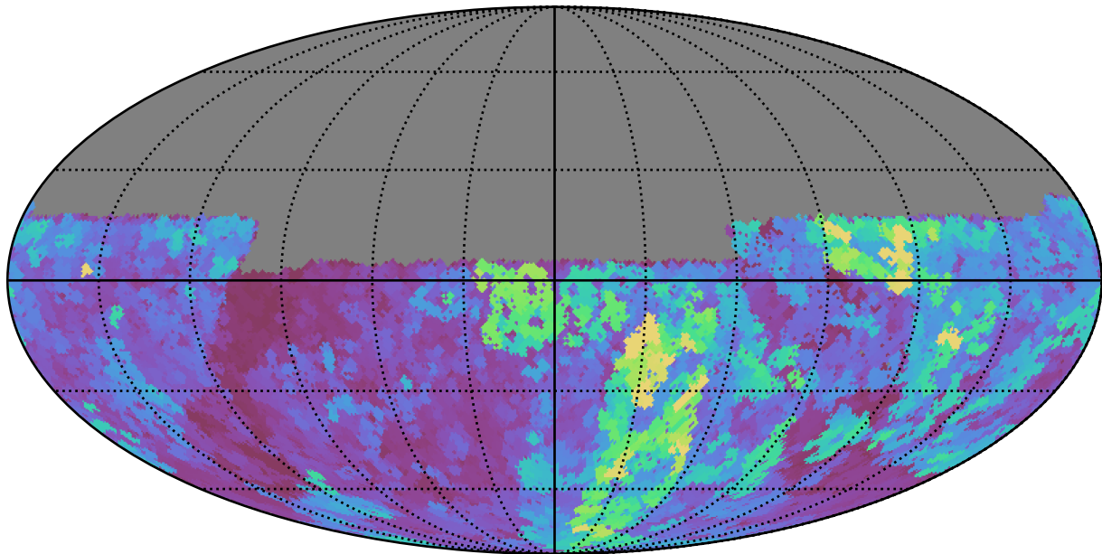
baseline_v2.1_10yrs Yr 1 y band: Max seeingEff
