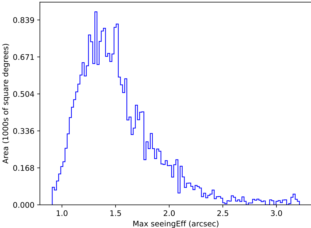
baseline_v2.1_10yrs Yr 1 r band: Max seeingEff
