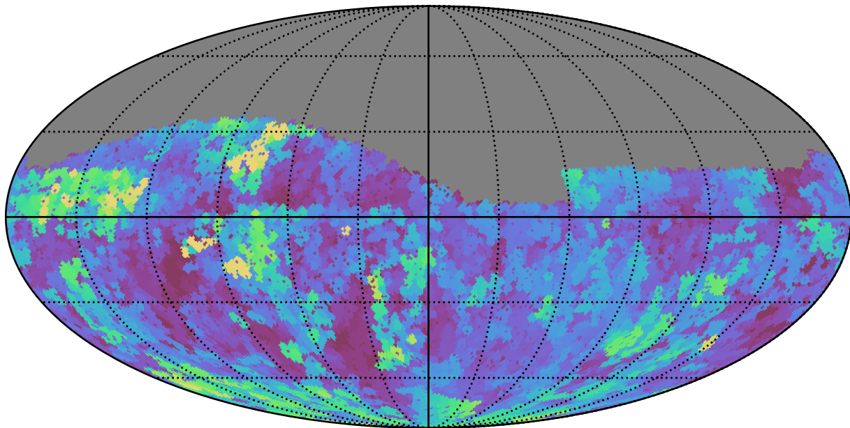
baseline_v2.1_10yrs Yr 1 g band: Max seeingEff
