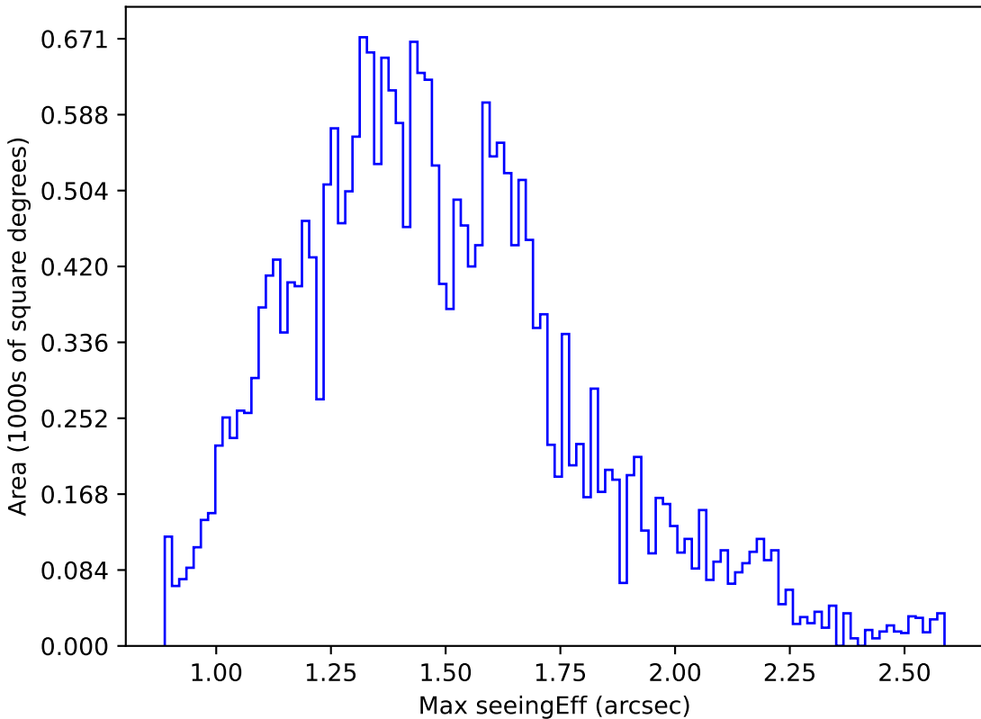
baseline_v2.1_10yrs Yr 1 g band: Max seeingEff
