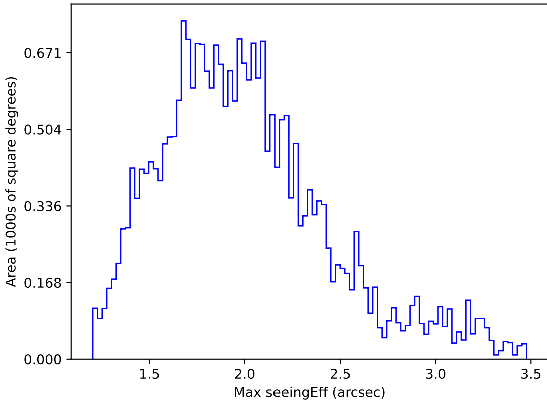
baseline_v2.1_10yrs Yr 1 all bands: Max seeingEff
