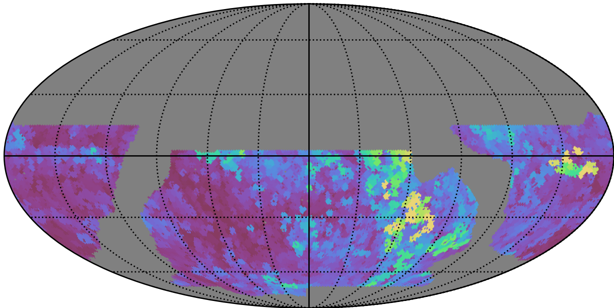
baseline_v2.1_10yrs WFD z band: Max seeingEff
