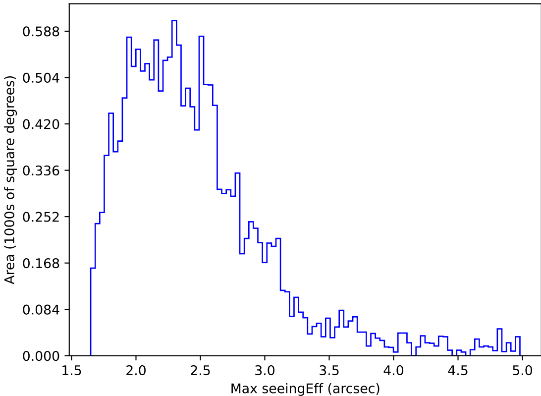
baseline_v2.1_10yrs WFD z band: Max seeingEff
