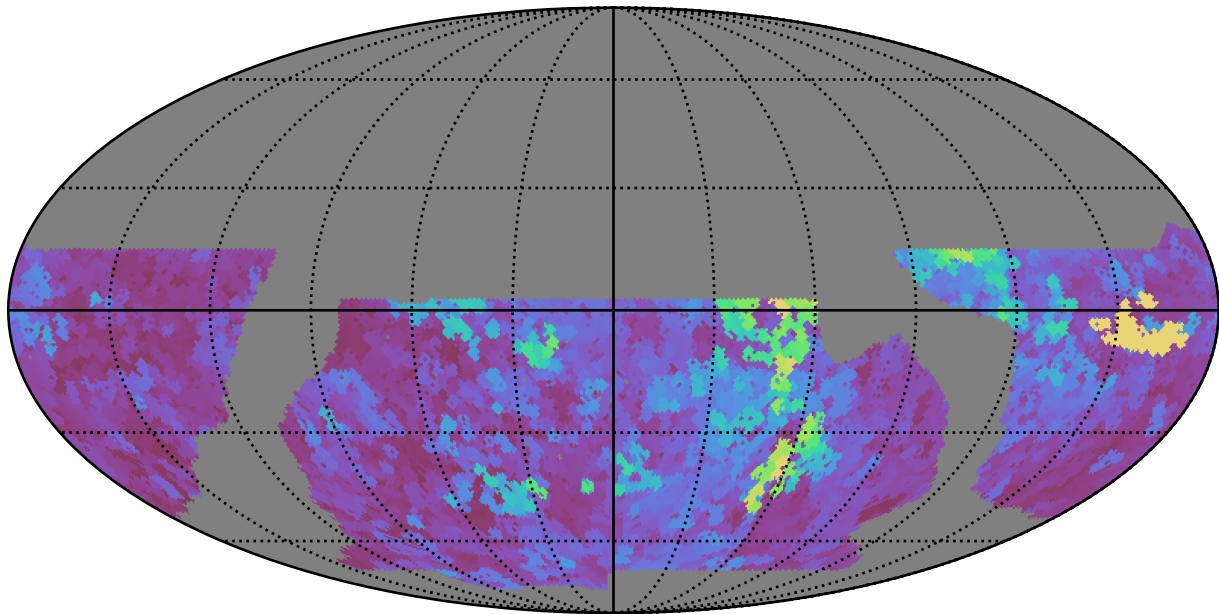
baseline_v2.1_10yrs WFD y band: Max seeingEff
