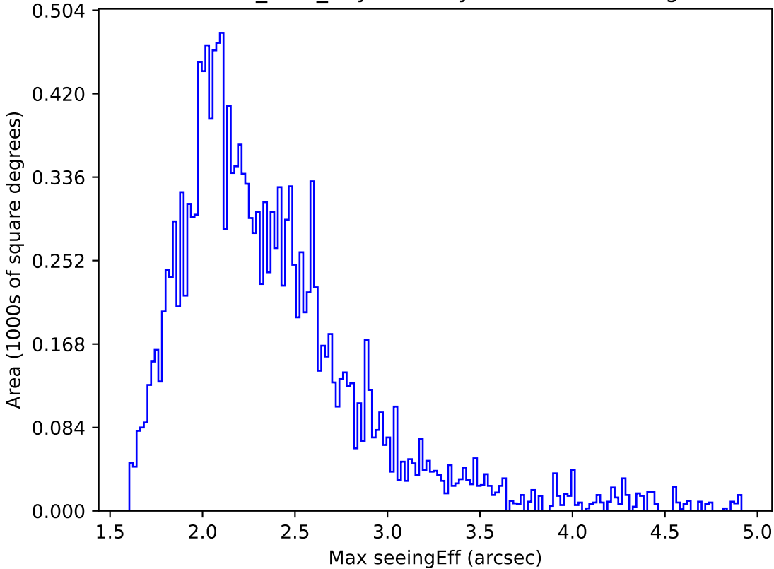
baseline_v2.1_10yrs WFD y band: Max seeingEff
