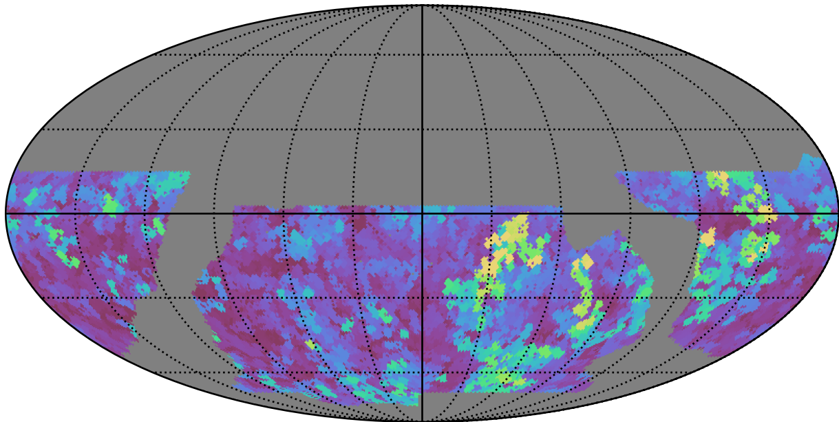
baseline_v2.1_10yrs WFD u band: Max seeingEff
