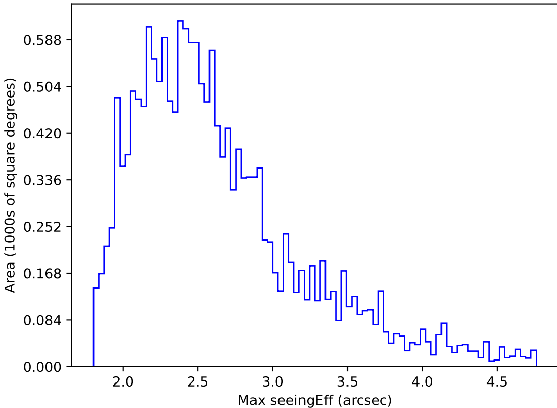
baseline_v2.1_10yrs WFD u band: Max seeingEff
