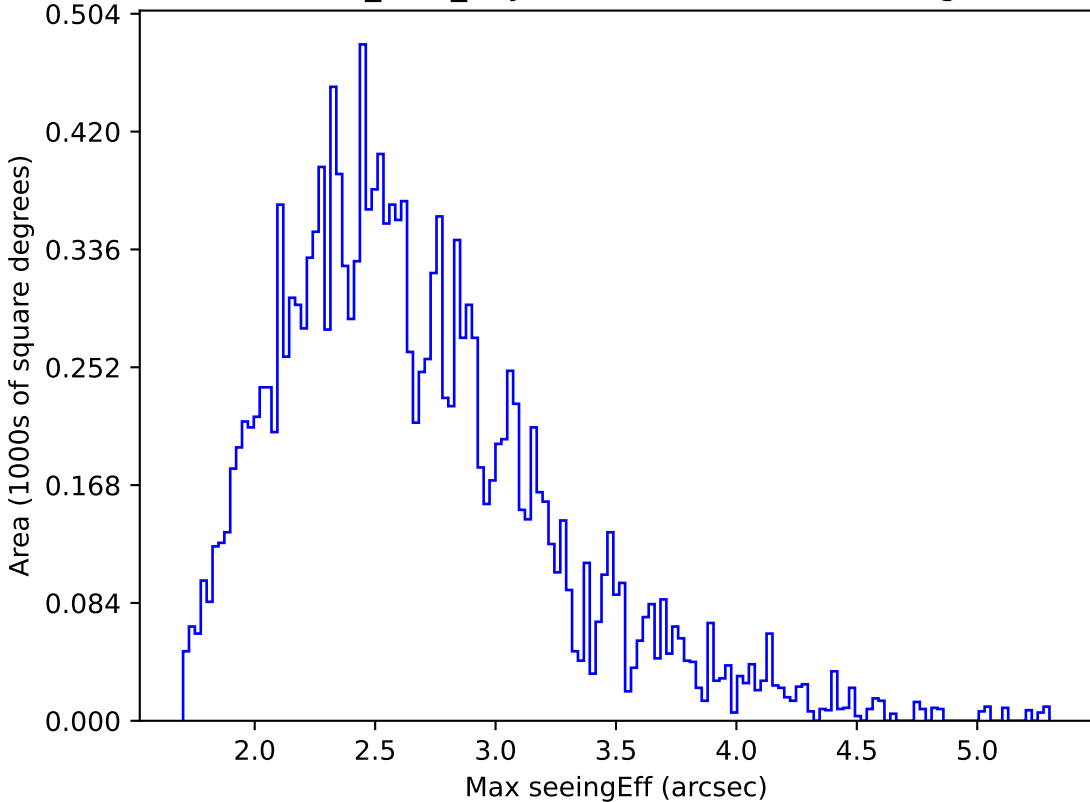
baseline_v2.1_10yrs WFD r band: Max seeingEff
