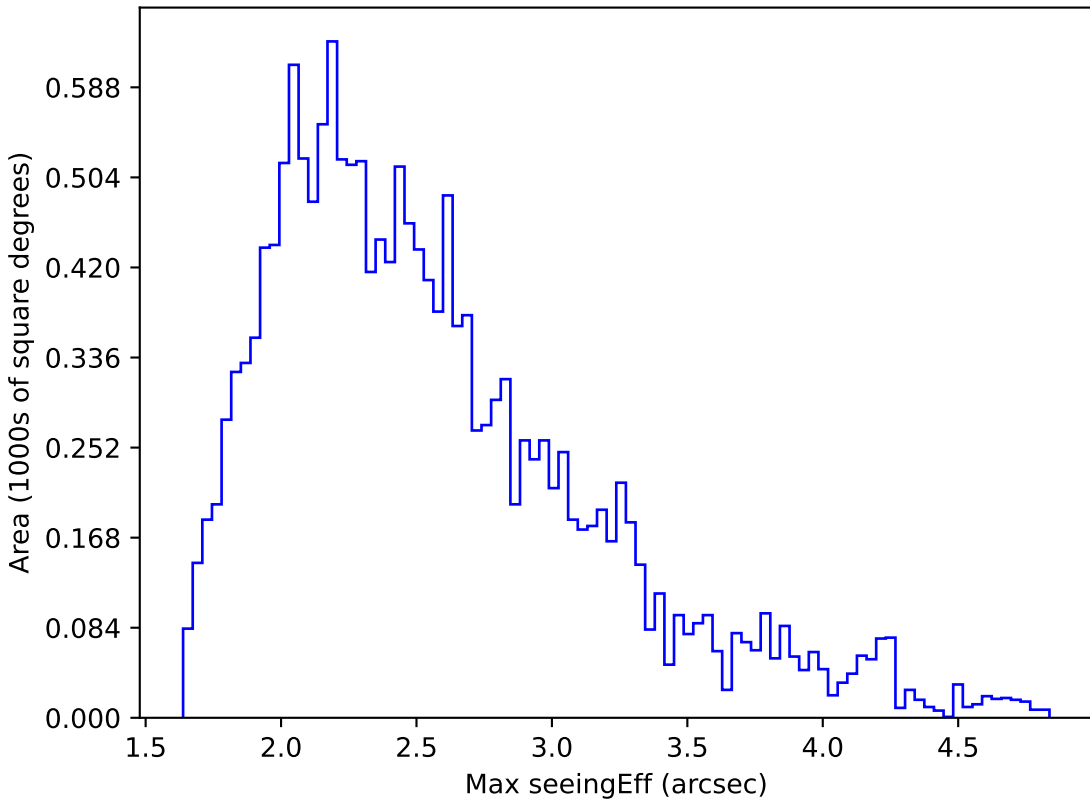
baseline_v2.1_10yrs WFD i band: Max seeingEff
