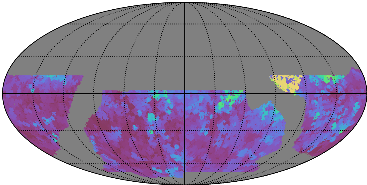
baseline_v2.1_10yrs WFD g band: Max seeingEff
