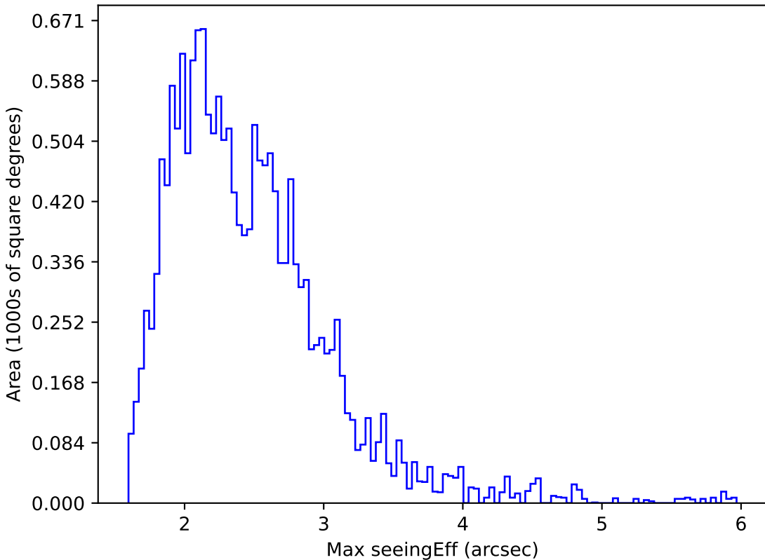
baseline_v2.1_10yrs WFD g band: Max seeingEff
