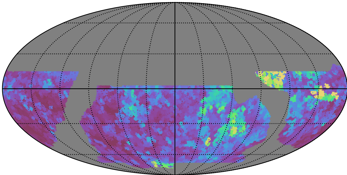
baseline_v2.1_10yrs WFD all bands: Max seeingEff
