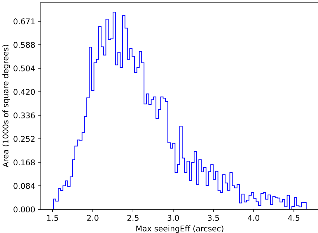
baseline_v2.1_10yrs All sky u band: Max seeingEff
