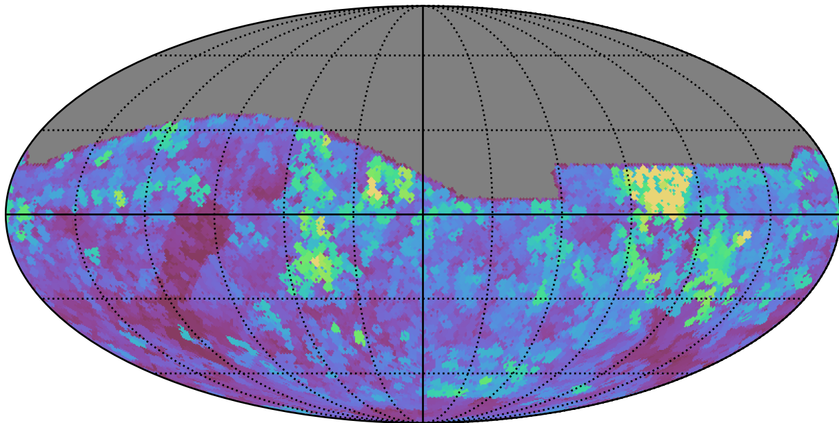
baseline_v2.1_10yrs All sky r band: Max seeingEff
