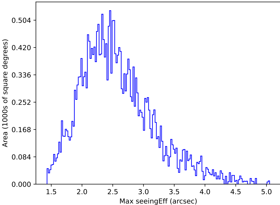
baseline_v2.1_10yrs All sky r band: Max seeingEff
