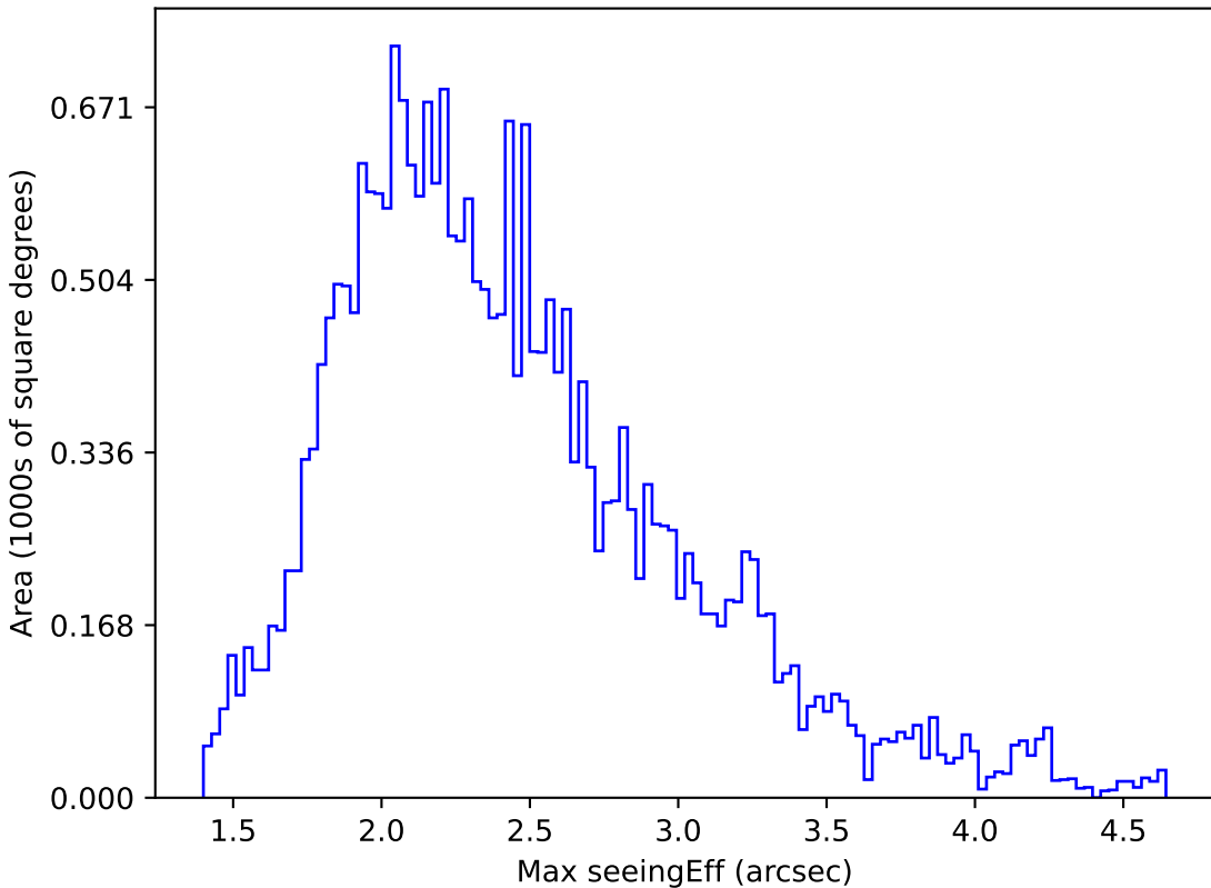
baseline_v2.1_10yrs All sky i band: Max seeingEff
