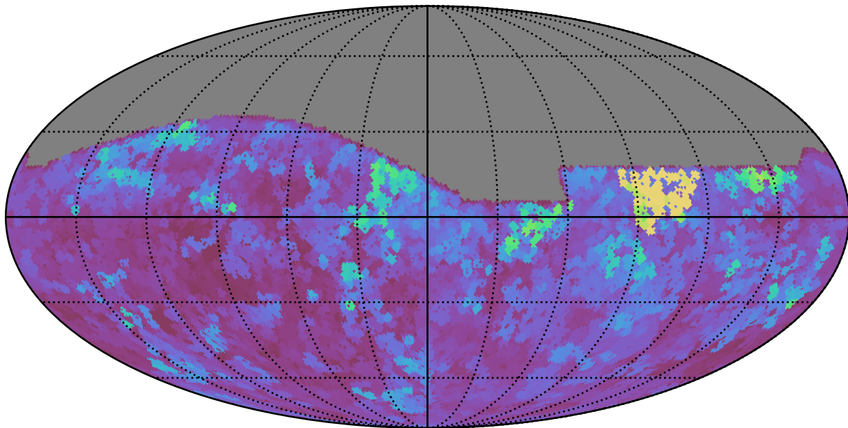
baseline_v2.1_10yrs All sky g band: Max seeingEff
