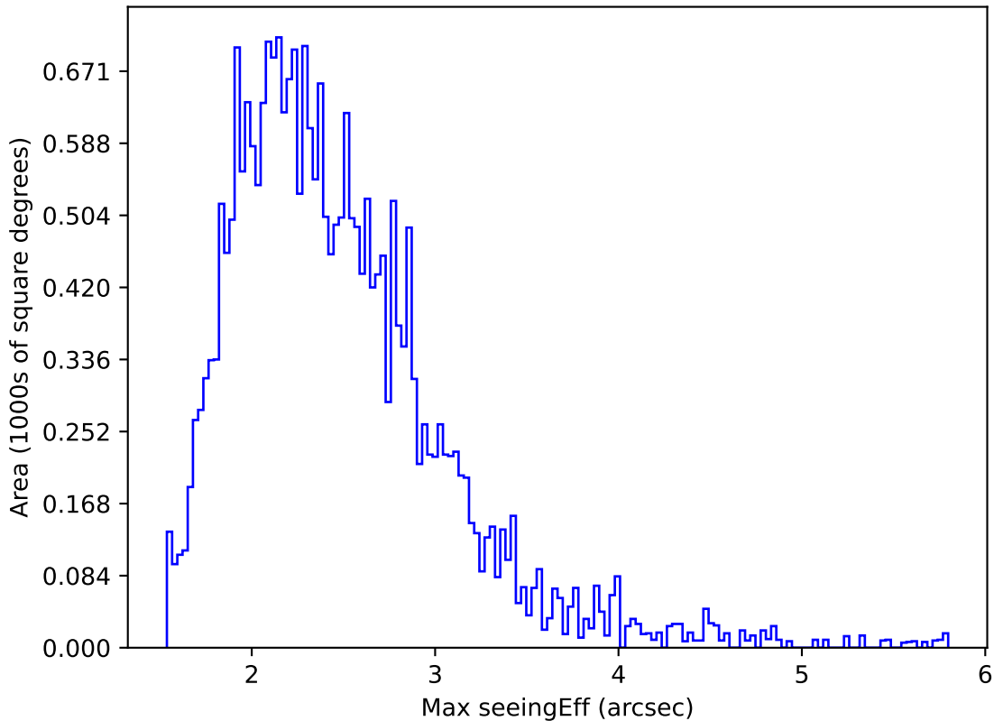
baseline_v2.1_10yrs All sky g band: Max seeingEff
