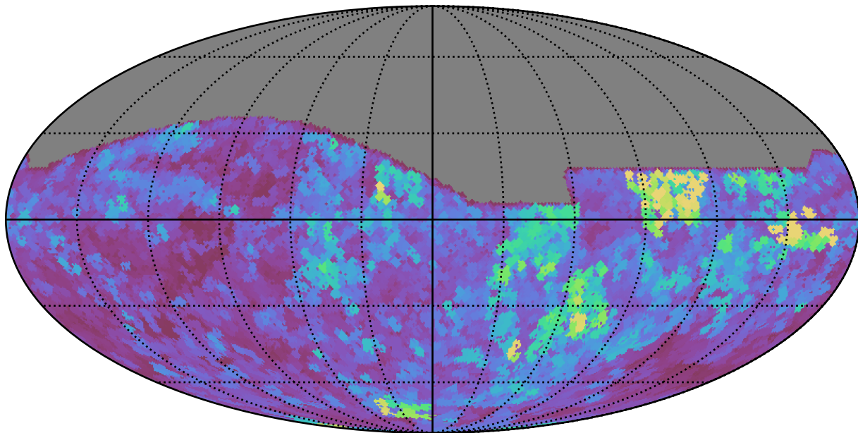
baseline_v2.1_10yrs All sky all bands: Max seeingEff
