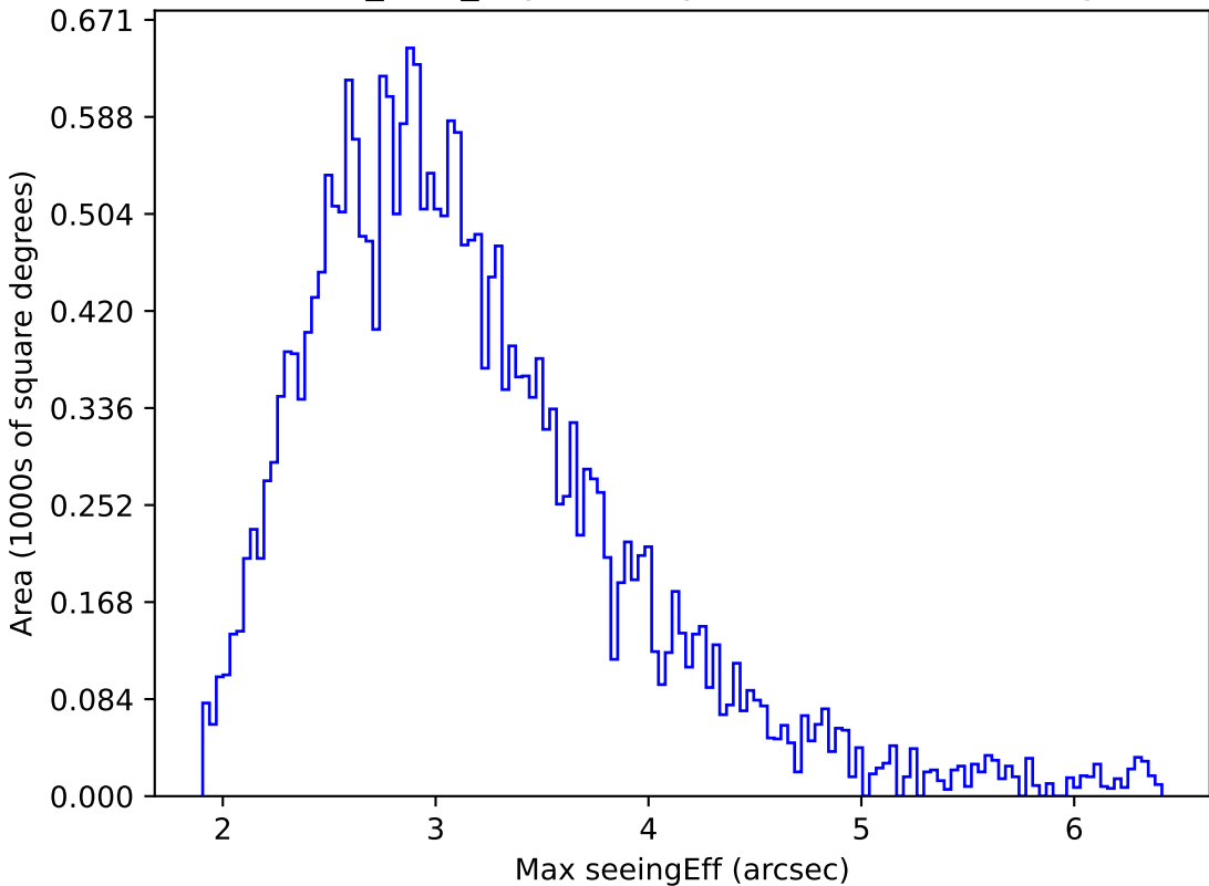
baseline_v2.1_10yrs All sky all bands: Max seeingEff
