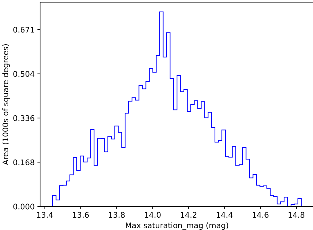
baseline_v2.1_10yrs WFD u band: Max saturation_mag
