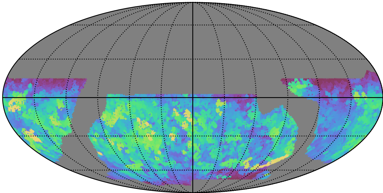
baseline_v2.1_10yrs WFD r band: Max saturation_mag
