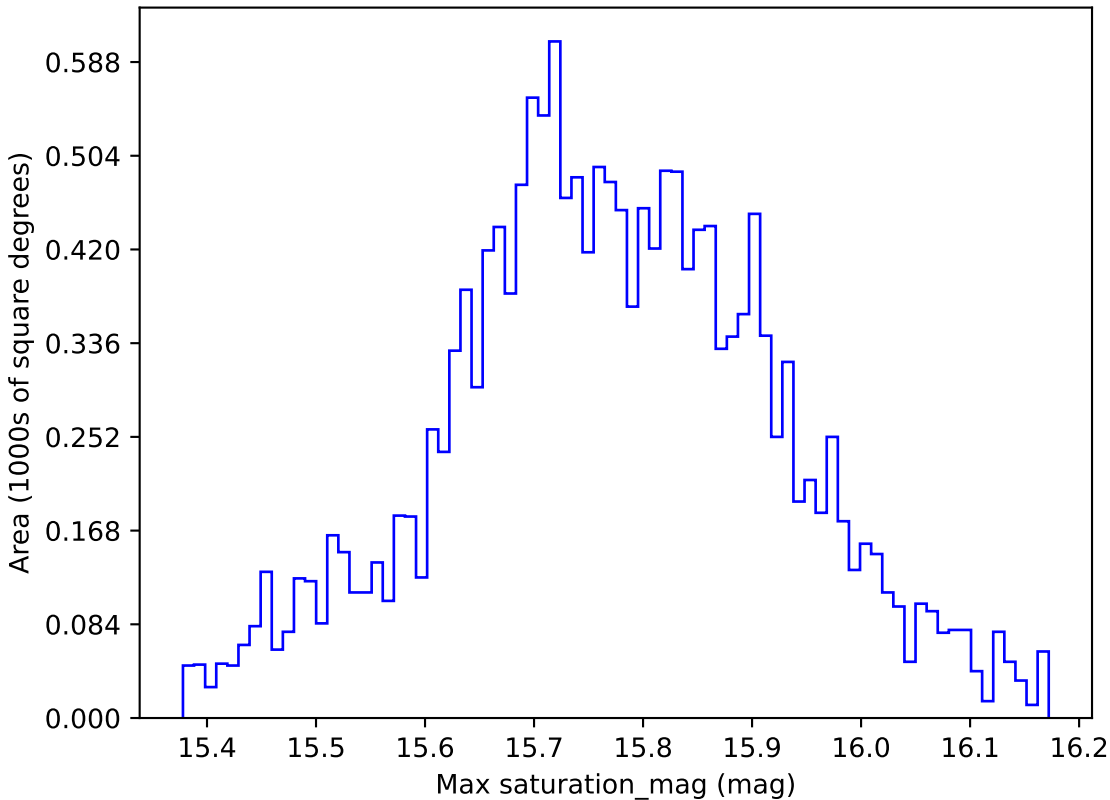
baseline_v2.1_10yrs WFD r band: Max saturation_mag
