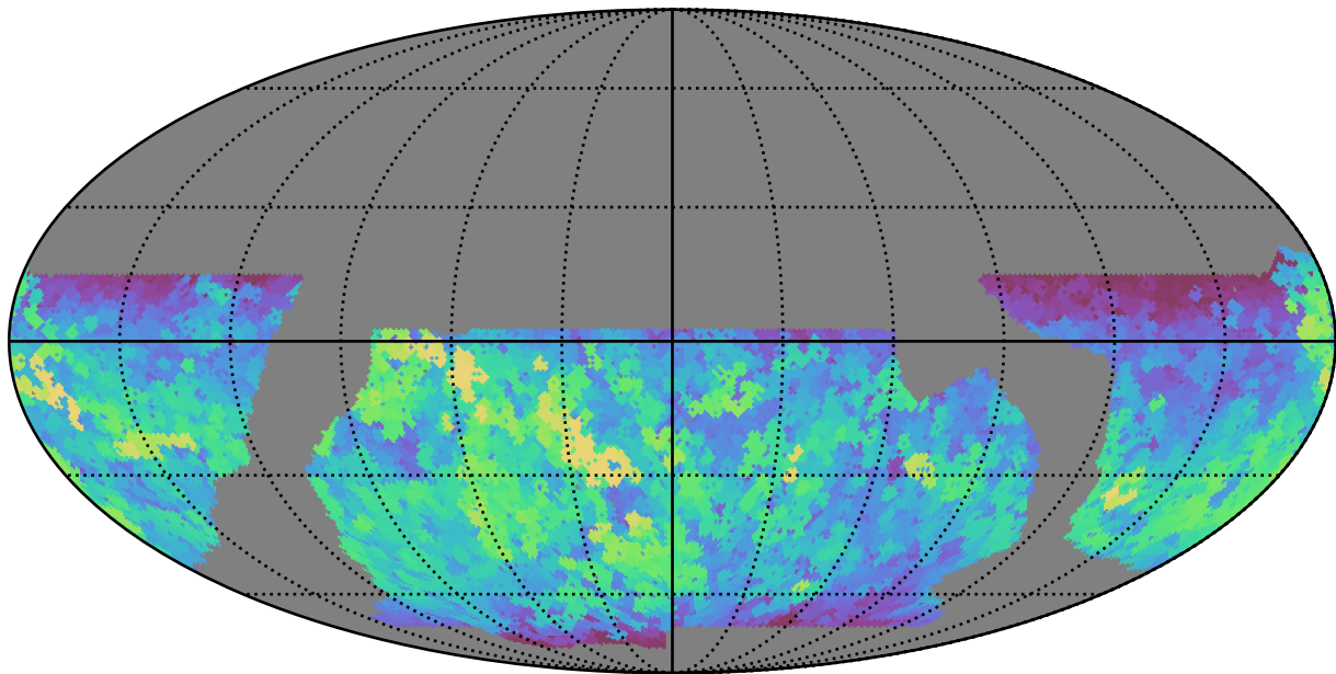
baseline_v2.1_10yrs WFD i band: Max saturation_mag
