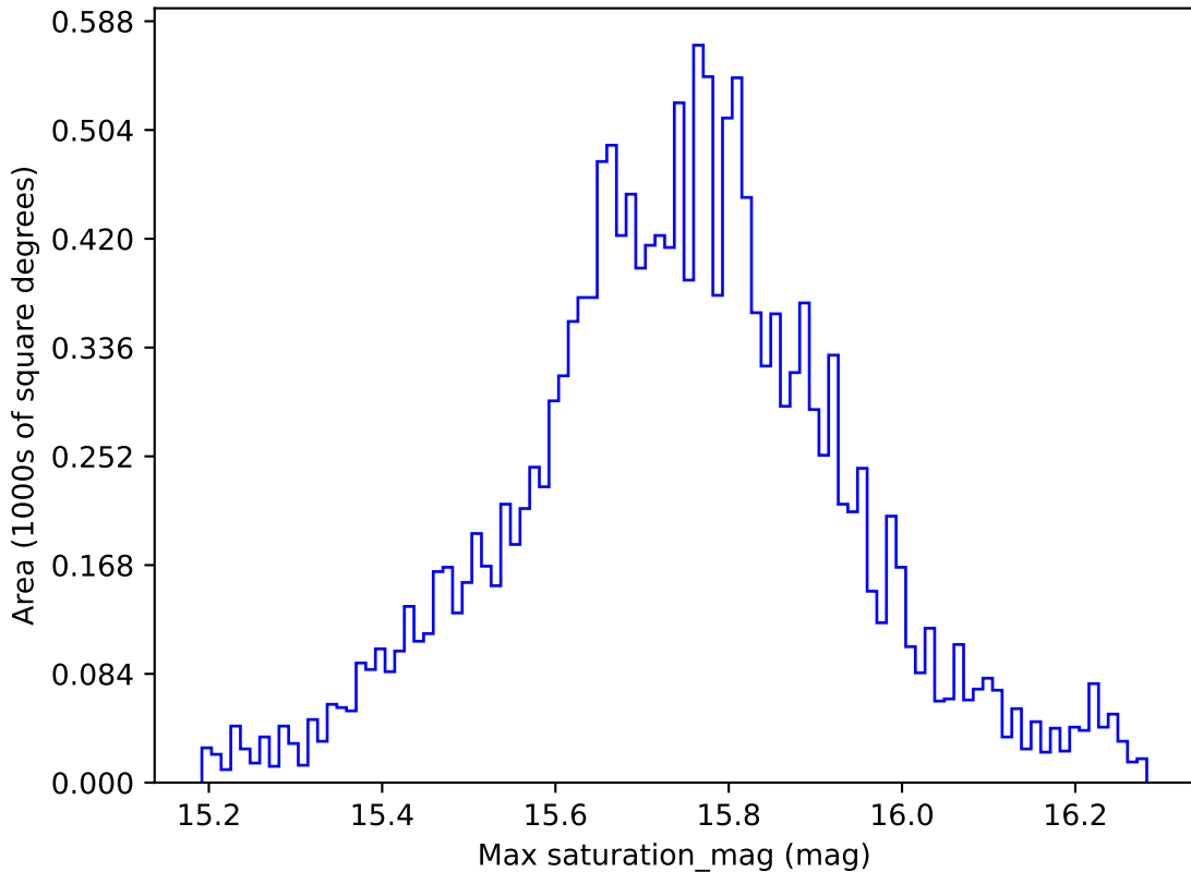
baseline_v2.1_10yrs WFD g band: Max saturation_mag
