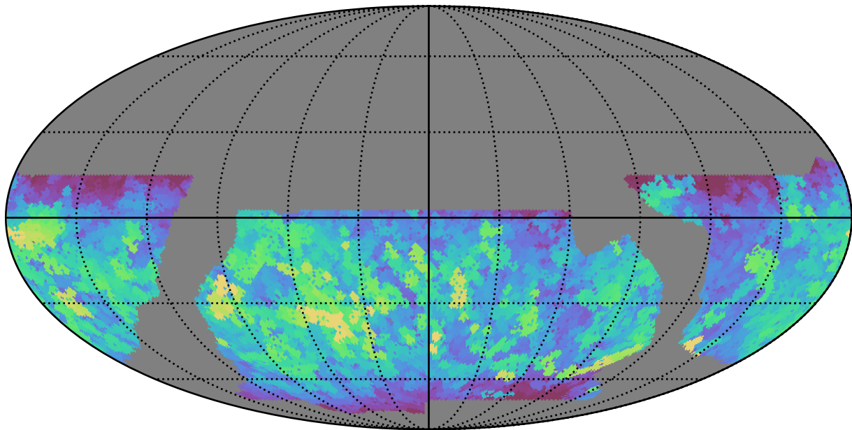
baseline_v2.1_10yrs WFD all bands: Max saturation_mag
