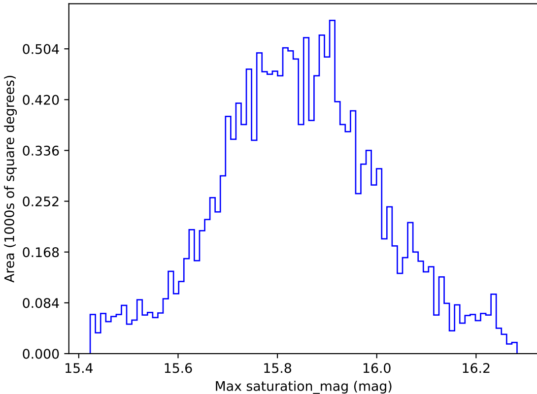
baseline_v2.1_10yrs WFD all bands: Max saturation_mag
