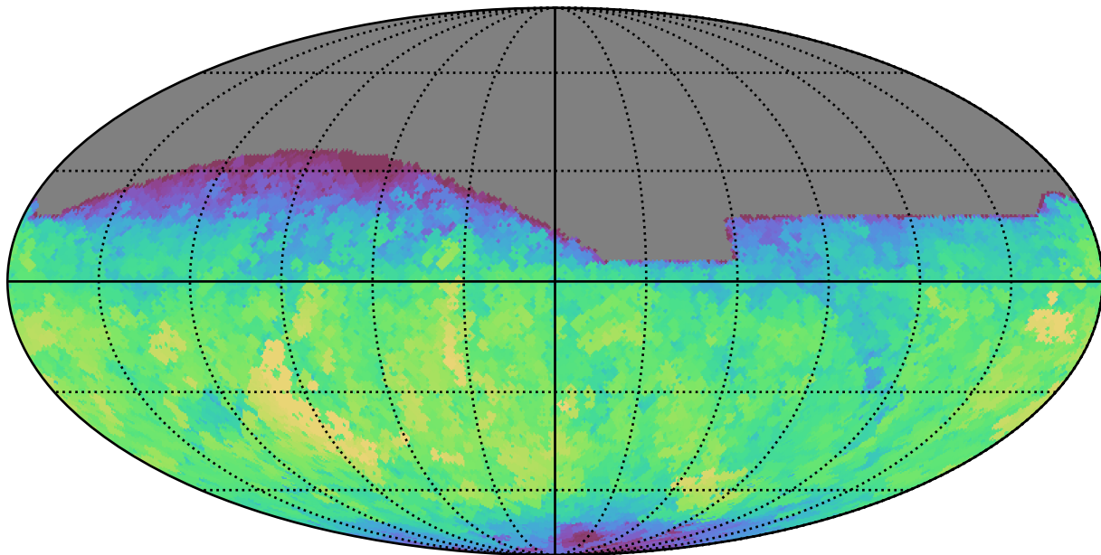
baseline_v2.1_10yrs All sky z band: Max saturation_mag
