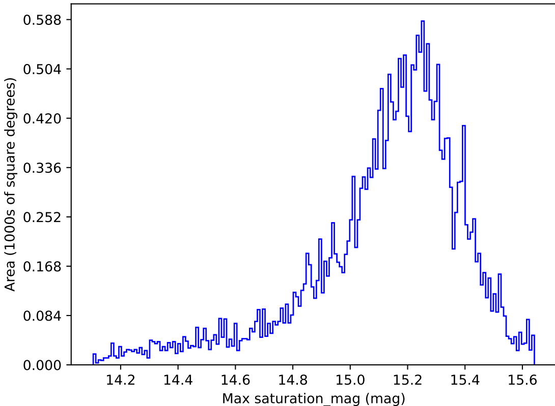
baseline_v2.1_10yrs All sky z band: Max saturation_mag
